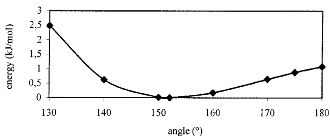
Figure 6. Bending potential curve for syn/syn Yb(SH) 2 at the MP2/6–31+G** level of theory
