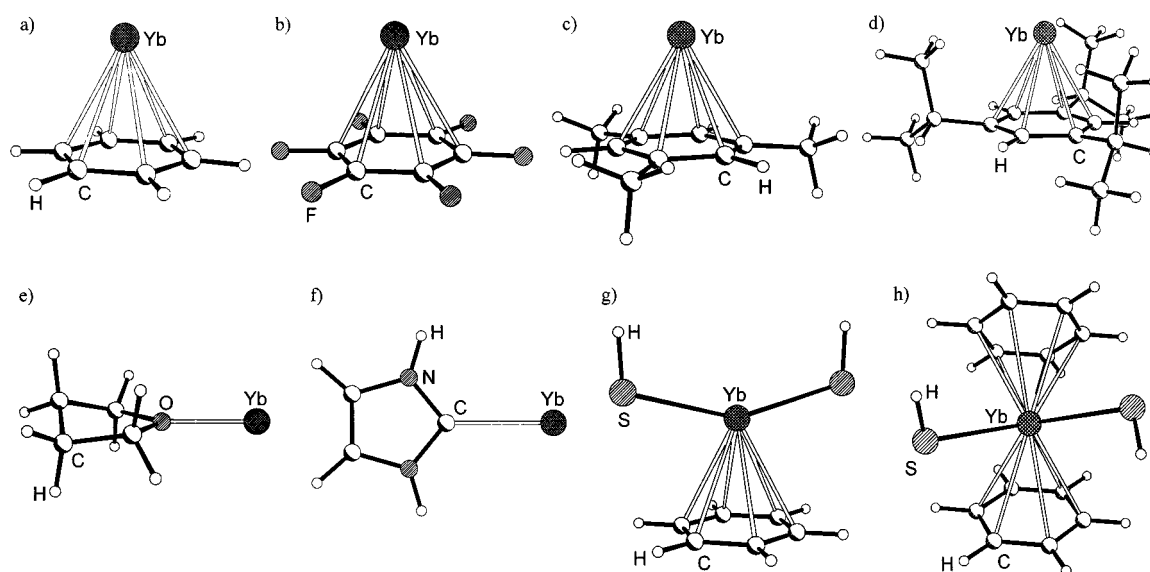
Figure 5. Optimized structures for the model compounds (a) [Yb(C 6 H 6 )] 2+ , (b) [Yb(C 6 F 6 )] 2+ , (c) [Yb(1,3,5-Me 3 C 6 H 3 )] 2+ , (d) [Yb(1,3,5- i Pr 3 C 6 H 3 )] 2+ , (e) [Yb(THF)] 2+ , (f) [Yb(imidazol-2-ylidene)] 2+ , (g) [Yb(SH) 2 (C 6 H 6 )], and (h) [Yb(SH) 2 (C 6 H 6 ) 2 ]; calculations were either performed at the B3LYP/6–31G* [(a)–(f)] or the MP2/6–31G* [(g), (h)] level of theory
