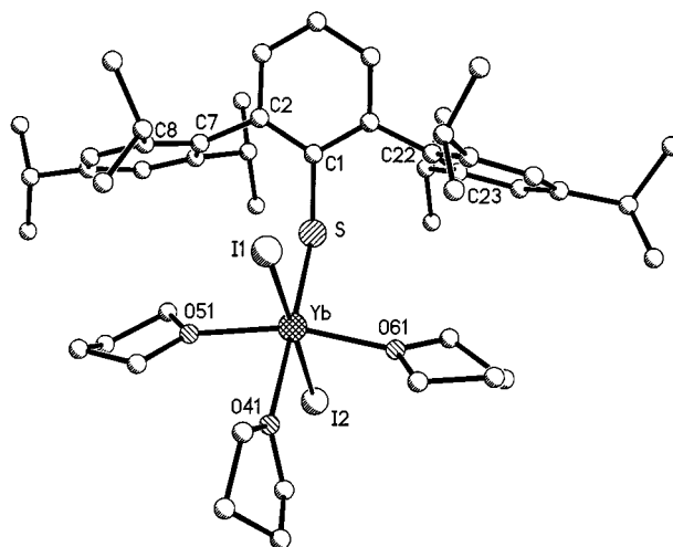
Figure 1. Molecular structure of 3 , showing the atom numbering scheme; hydrogen atoms have been omitted for clarity
