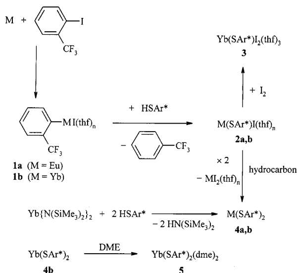
Scheme 1. Syntheses of compounds 1 – 5
