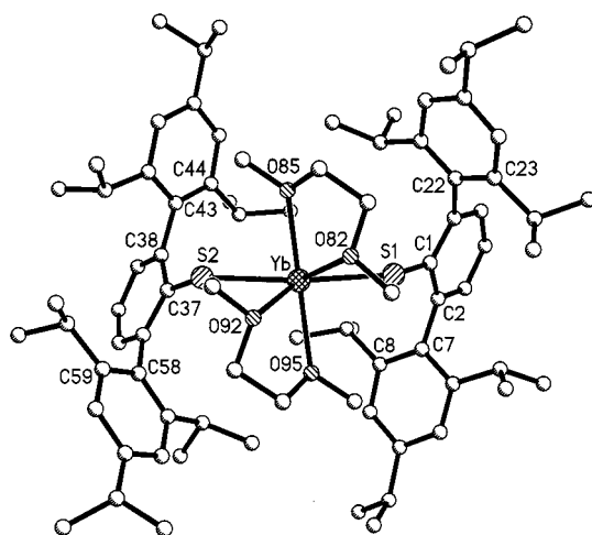
Figure 4. Molecular structure of 5 , showing the atom numbering scheme; hydrogen atoms and the minor parts of the disordered isopropyl groups have been omitted for clarity
